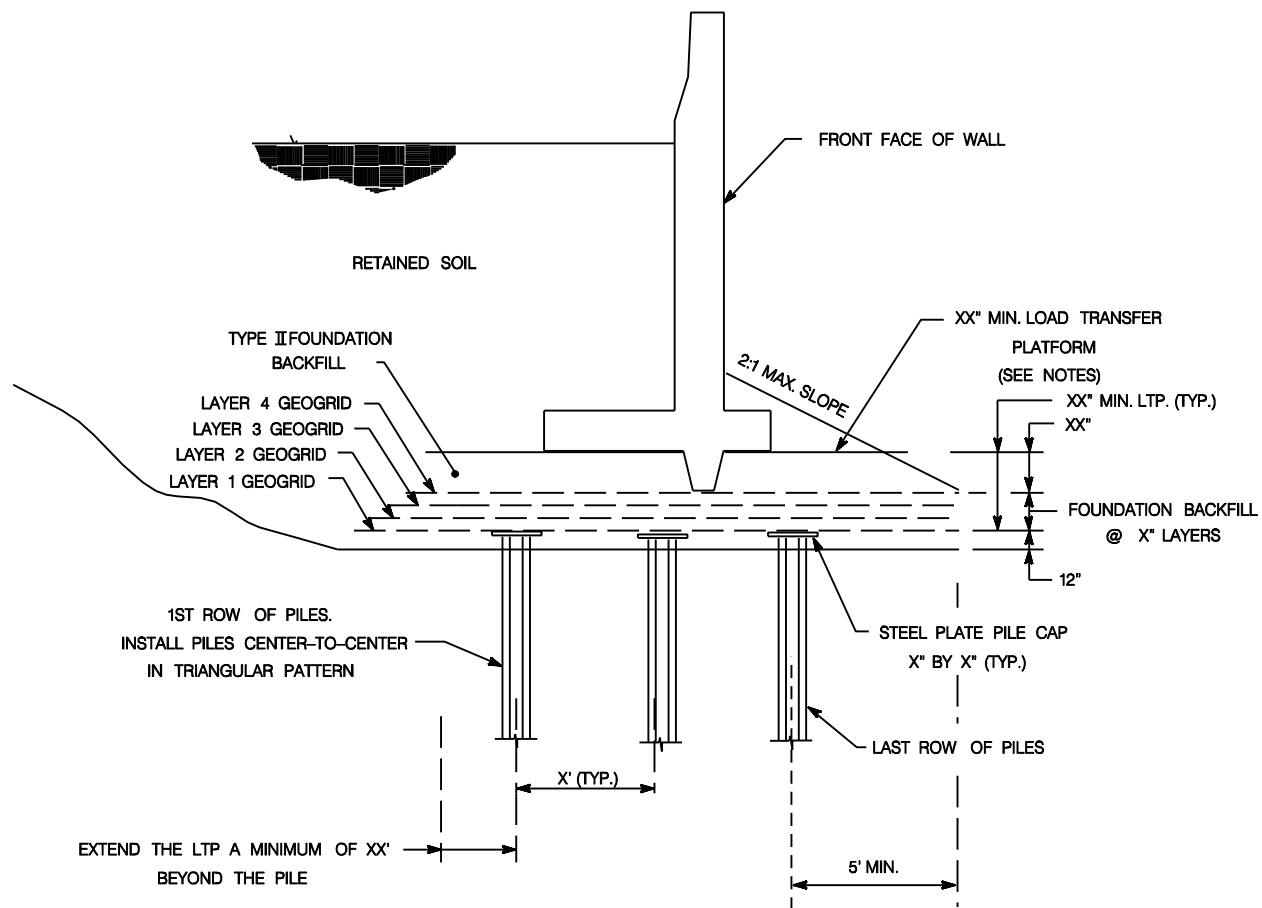
CANTILEVER WALL WITH KEY
