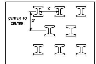
PILES CENTER-TO-CENTER IN TRIANGULAR PATTERN
